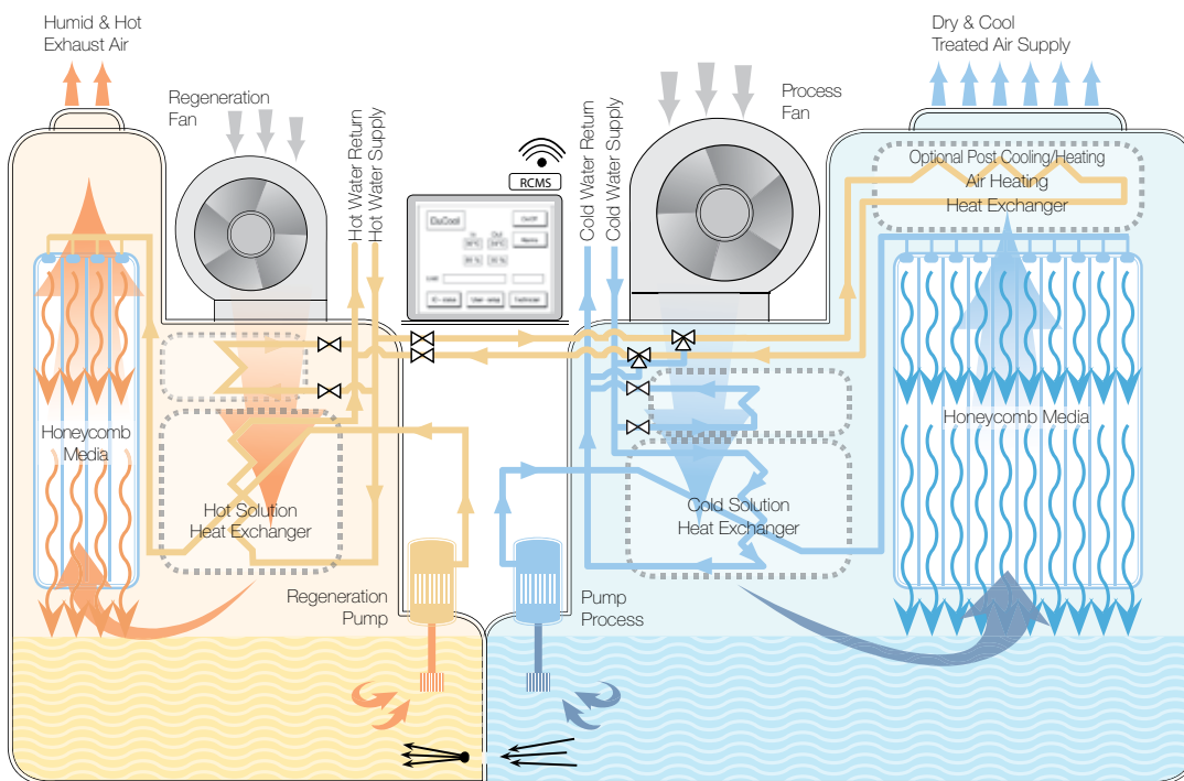
Schematic Process Diagram
